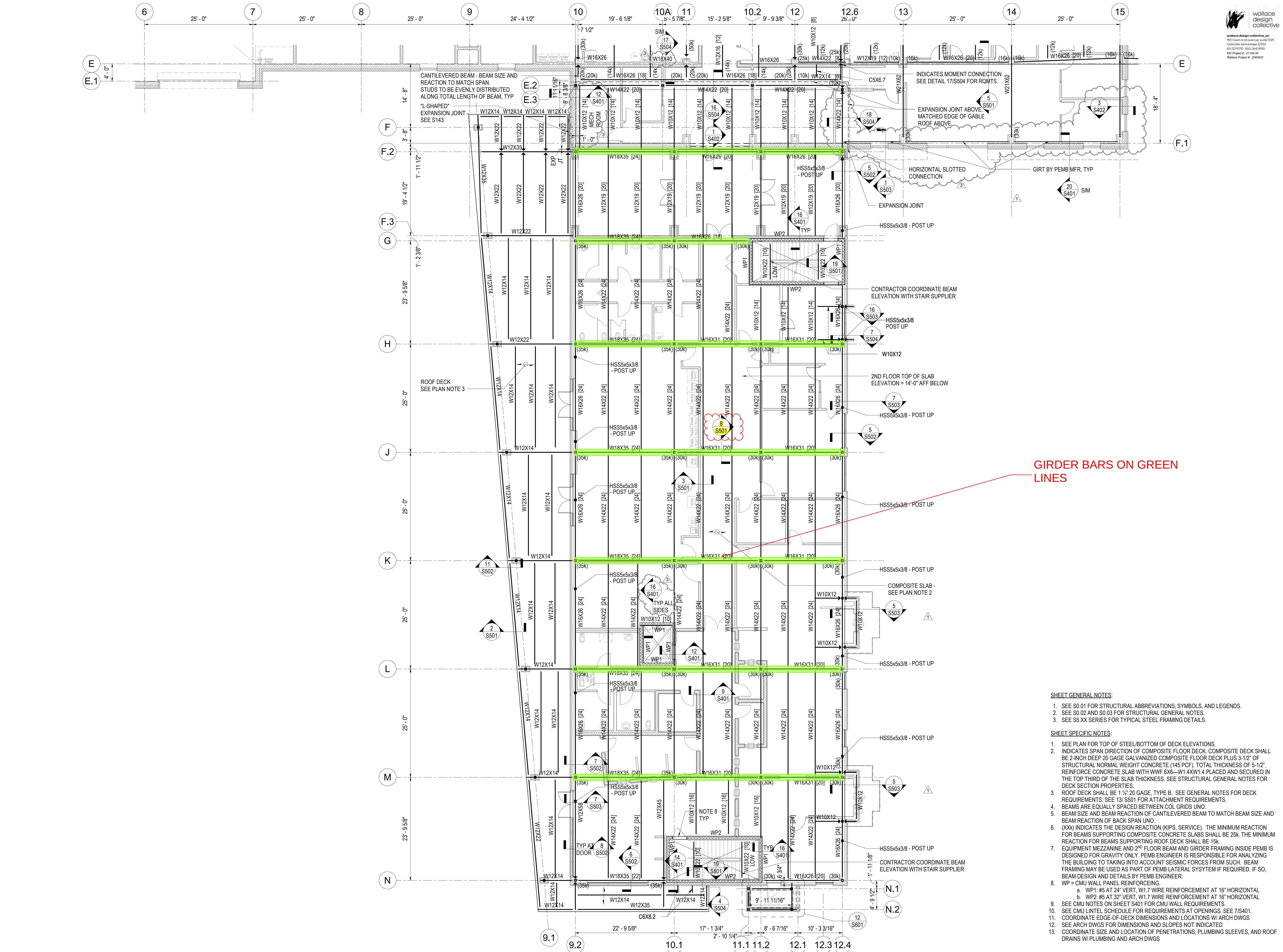
1 PARTIAL SECOND FLOOR FRAMING PLAN - AREA 'C'
