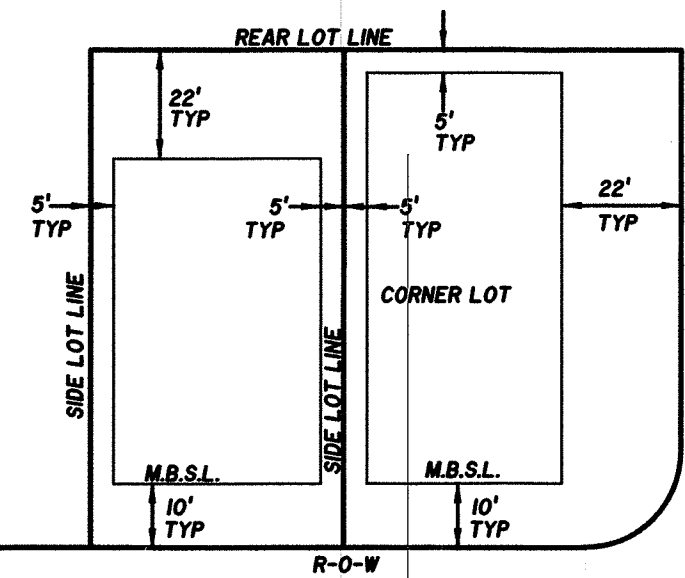
TYPICAL MINIMUM BUILDING SETBACKS N.T.S.
